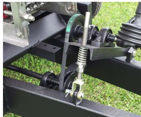
Belt driven drive shaft for spinners with PTO shaft and adjustable tensioner.
