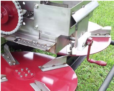
Stainless steel adjustable slide for pattern accuracy and adjustment
